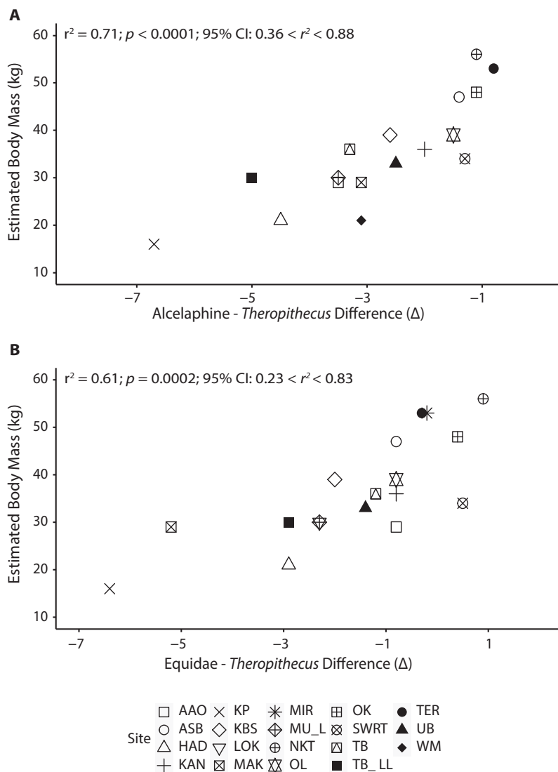
Fig. 4. Larger species of Theropithecus engaged in greater bulk-feeding behavior. Median body mass of Theropithecus in a given assemblage plotted as a function of mean difference ( \Delta ) in \delta^{13}\text{C} values between it and coeval (A) alcelaphines and (B) equids. Key to STU names: AAO: Ahl al Oughlam; ASB: Asbole; HAD: Hadar (SHM, DDM, KHM); KAN: Kanjera South; KP: Kanapoi; KBS: KBS, Koobi Fora; LOK: Lokochot, Koobi Fora; MAK: Makapansgat; MIR: Mirzapur, Indian Siwaliks; MU_L: Middle and Upper Lomekwi, Nachukui; NKT: Nariokotome, Nachukui; OL: Olduvai Gorge; OK: Okote, Koobi Fora; SWRT: Swartkrans; TB: Tulu Bor, Koobi Fora ( T. darti ); TB_LL: Tulu Bor, Koobi Fora / Lower Lomekwi, Nachukui ( T. brumpti ); TER: Tighennif; UB: Upper Burgi, Koobi Fora; WM: Woranso-Mille.
