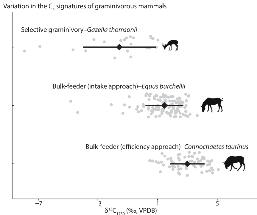
Fig. 1. Selective graminivores such as Gazella thomsonii are often depleted in ^{13}\text{C} relative to bulk-feeding graminivores such as Connochaetes taurinus and Equus burchellii inhabiting the same ecosystem. Data source: Cerling et al. (2015), but \delta^{13}\text{C} values are adjusted to reflect pre-industrial levels of atmospheric \text{CO}_2 .
